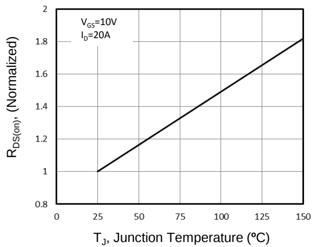
Figure 7. Drain-Source On-Resistance
